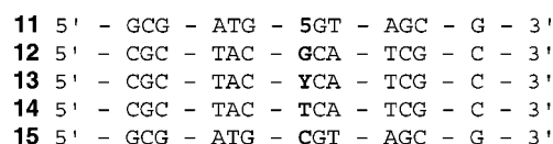
Figure 5. Oligonucleotide sequences where Y = 8-oxoG.
